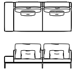
S-644L 2人掛け片肘ソファ W2340×D1065×H655×SH370
