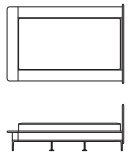
BE-131 single bed (Europe) W1520 × D2284 × H885 × MH525
