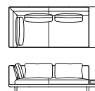
S-511RT corner sofa + side table W2330×D1020×H680×SH380
