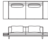
S-505RLT 2 seater sofa + arm + side table W2640 × D1020 × H680 × SH380
