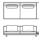
S-504RT 2 seater sofa + side table W2330×D1020×H680×SH380
