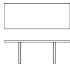
PZT-003 table (round legs) W2400×D850×H750
